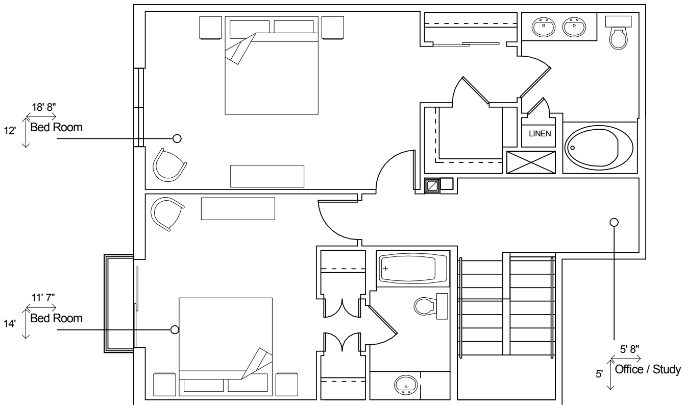
2nd Floor
